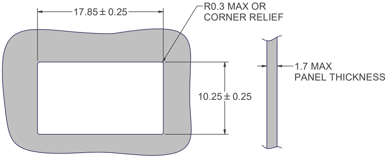
RECOMMENDED MOUNTING CUTOUT
